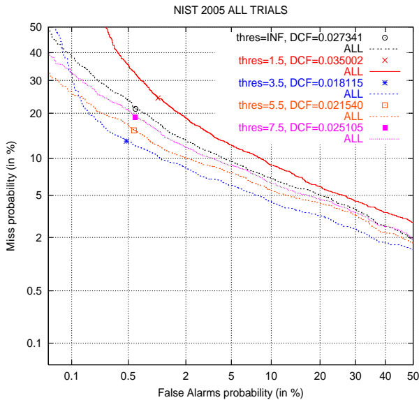
Fig. 1. DET curves for various adaptation thresholds used in the unsupervised speaker adaptation. Joint factor analysis with 25 channel factors. z -norm score normalization. All trials, male and female.
