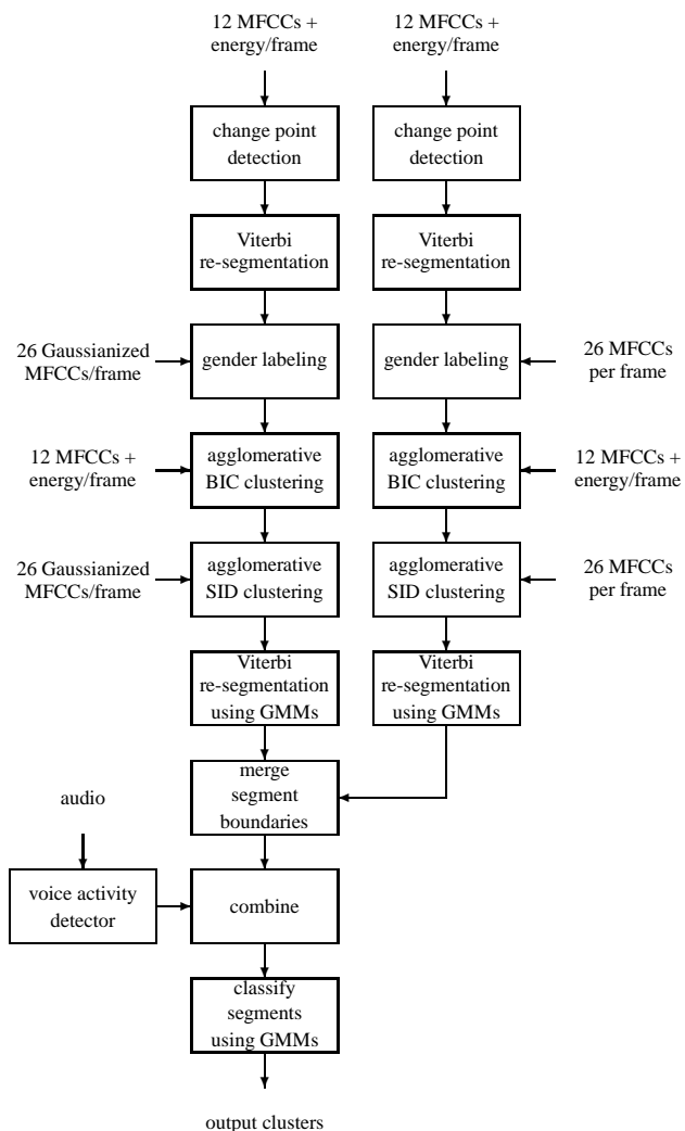
Fig. 1. Multistage speaker diarization algorithm combining clusters from Gaussianized and non-Gaussianized features.
