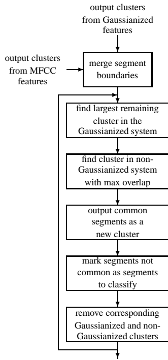
Fig. 2. Flowchart of process for combining clusters resulting from Gaussianized and non-Gaussianized systems.
