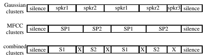
Fig. 3. Example showing combination of clusters from Gaussianized and non-Gaussianized (MFCC) systems. Segments marked X in the combined cluster are reclassified using adapted GMMs for S1, S2 and silence.
