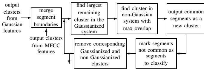
Fig. 2. Flowchart for combining clusters from Gaussianized and non-Gaussianized systems
