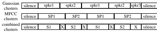
Fig. 3. Example showing combination of clusters from Gaussianized and non-Gaussianized (MFCC) systems. Segments marked X in the combined cluster are reclassified using adapted GMMs for S1 , S2 and silence.
